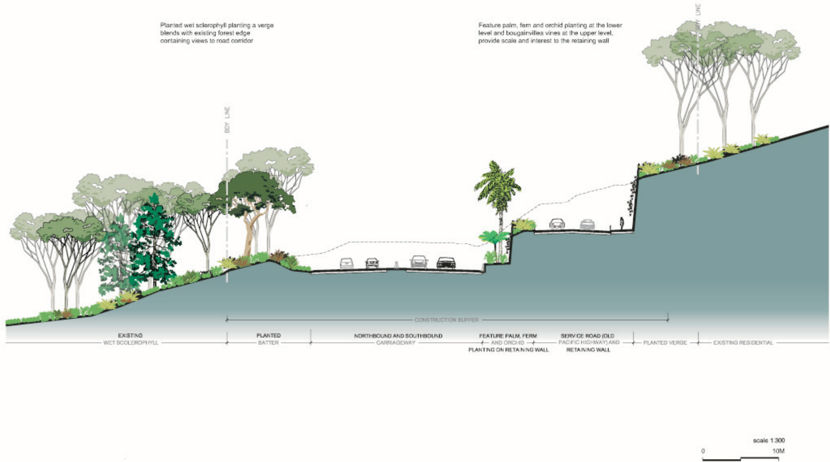
LS.6 Cross Section @ STN 45500
